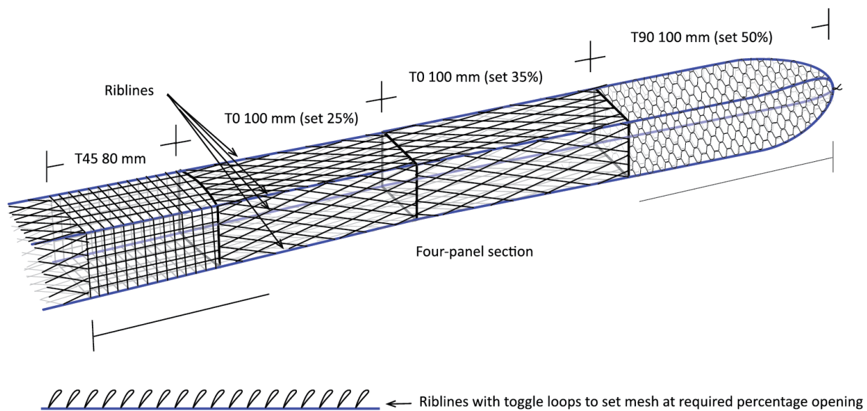
Figure 2. Diagram of test gear by Dr Matthew McHugh
